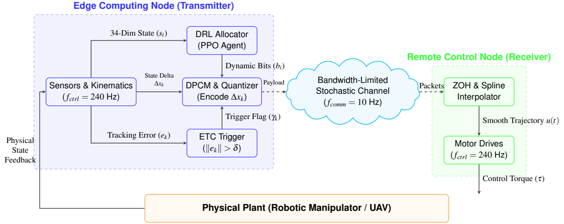
Figure 2: The proposed Joint Communication and Control (JCC) system architecture encompassing dual-frequency decoupling and network imperfections.
